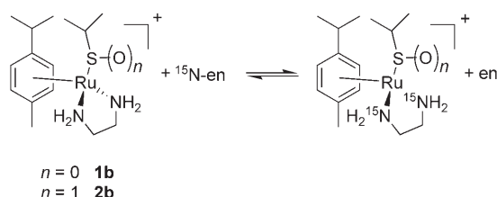
Scheme 2. Exchange of ethylenediamine is much faster for the thiolato complex 1b ( n=0 ) than for the sulfenato complex 2b ( n=1 ).
